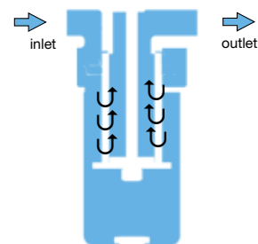
cross-section
